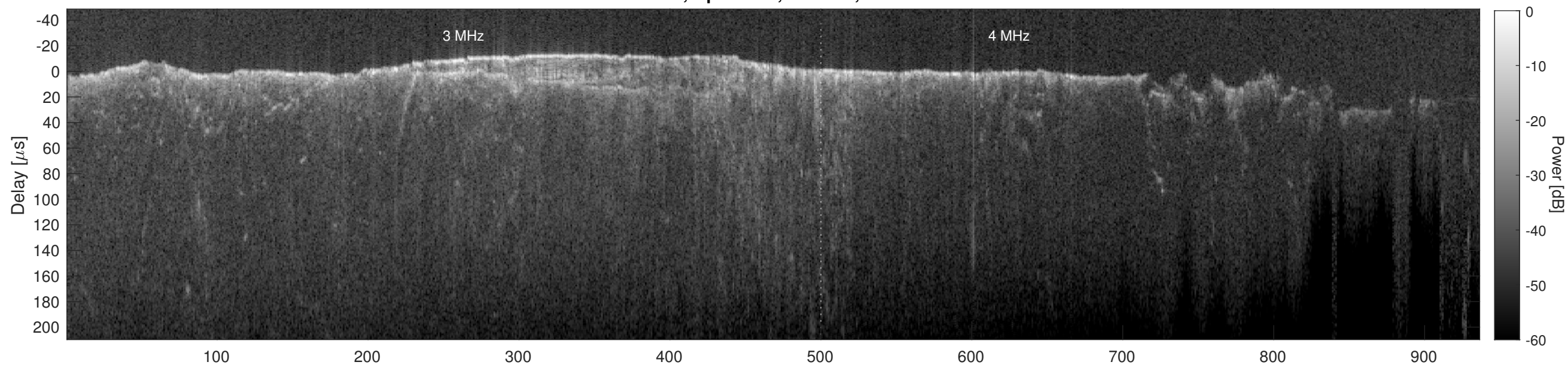
Orbit 8645, Cluttergram
