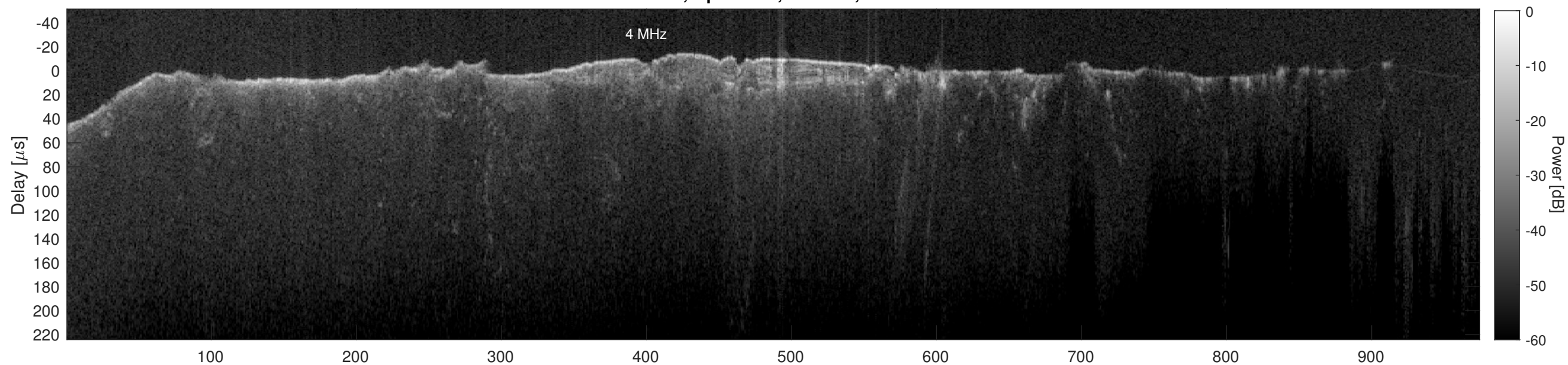
Orbit 8646, Cluttergram
