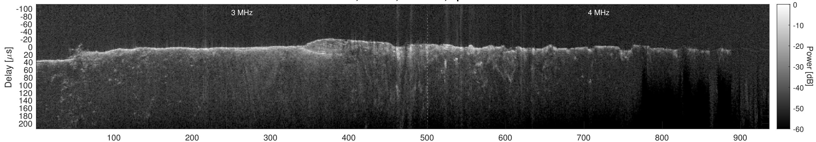
Orbit 8647, Cluttergram
