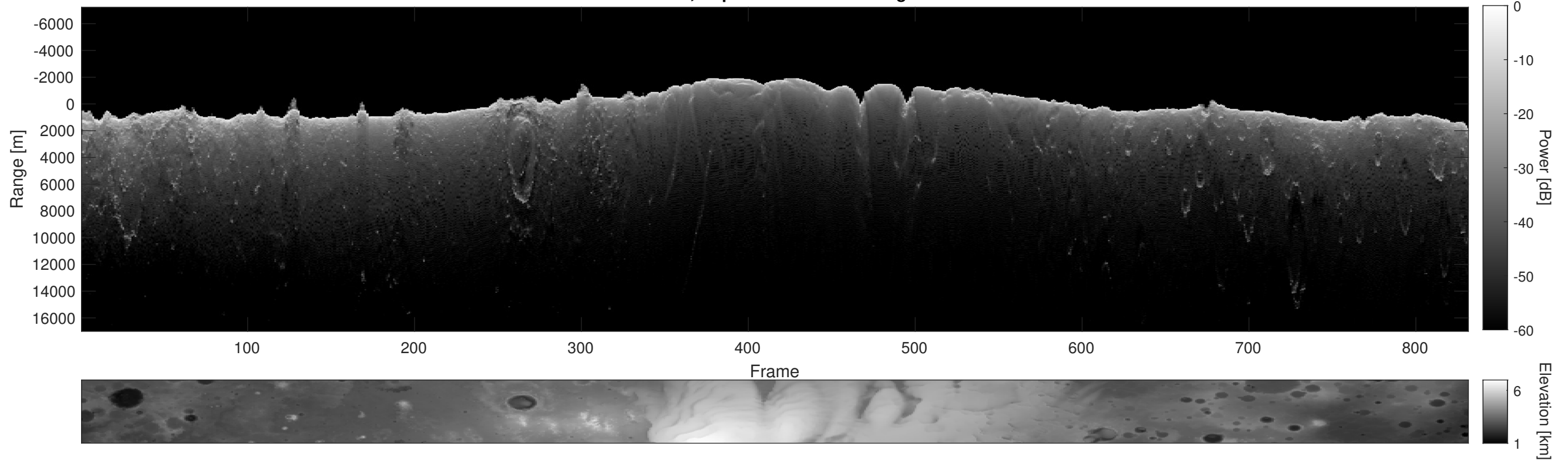
Orbit 8650, Depth-Corrected Cluttergram
