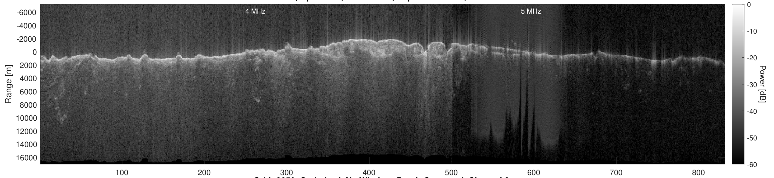
Orbit 8650, Optimized, No Window, Depth-Corrected, Channel 2
