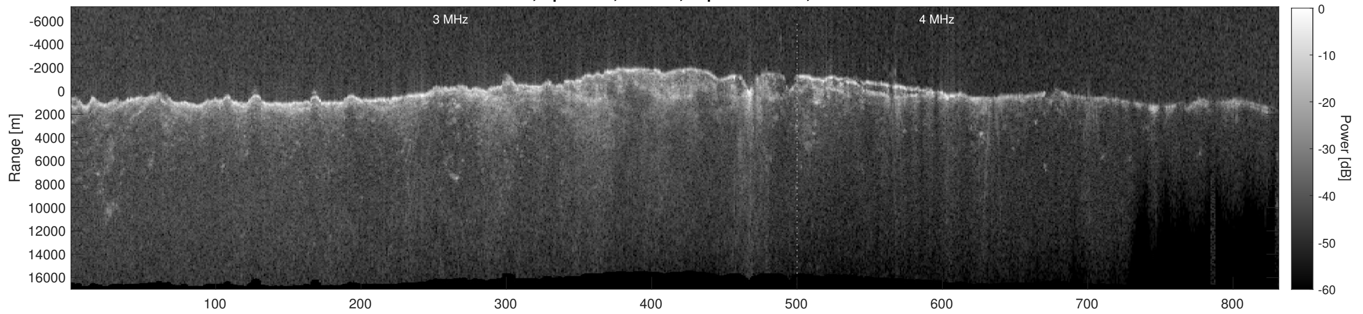
Orbit 8650, Depth-Corrected Cluttergram
