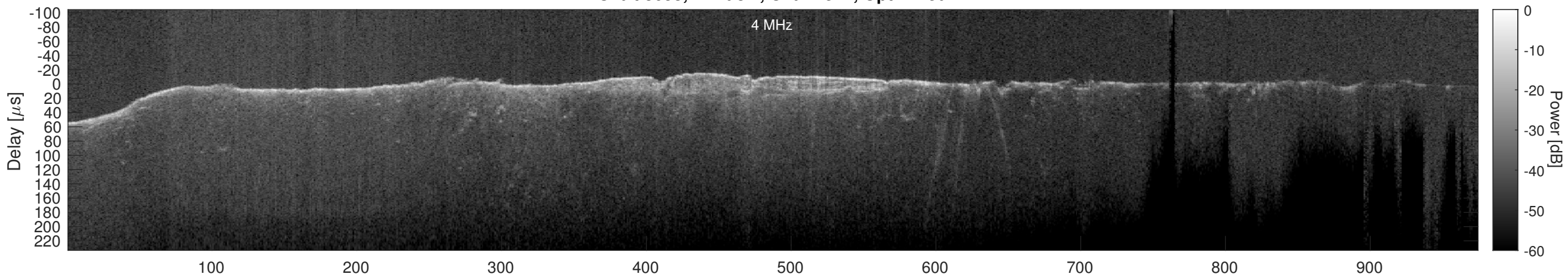
Orbit 8653, Cluttergram
