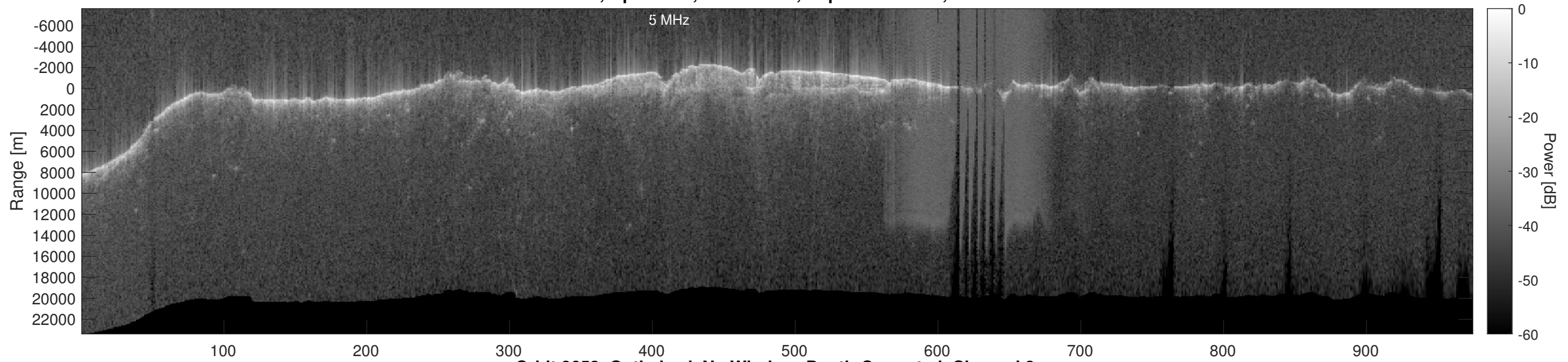
Orbit 8653, Optimized, No Window, Depth-Corrected, Channel 2
