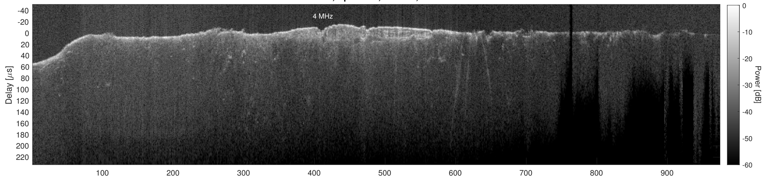
Orbit 8653, Cluttergram
