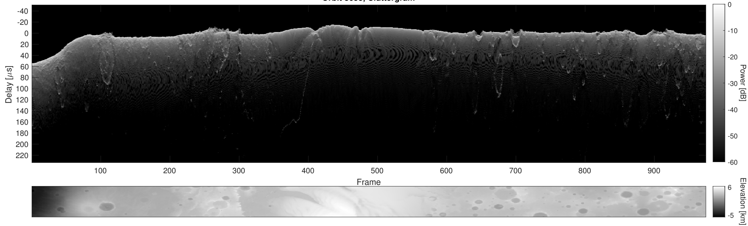
Orbit 8653, Cluttergram
