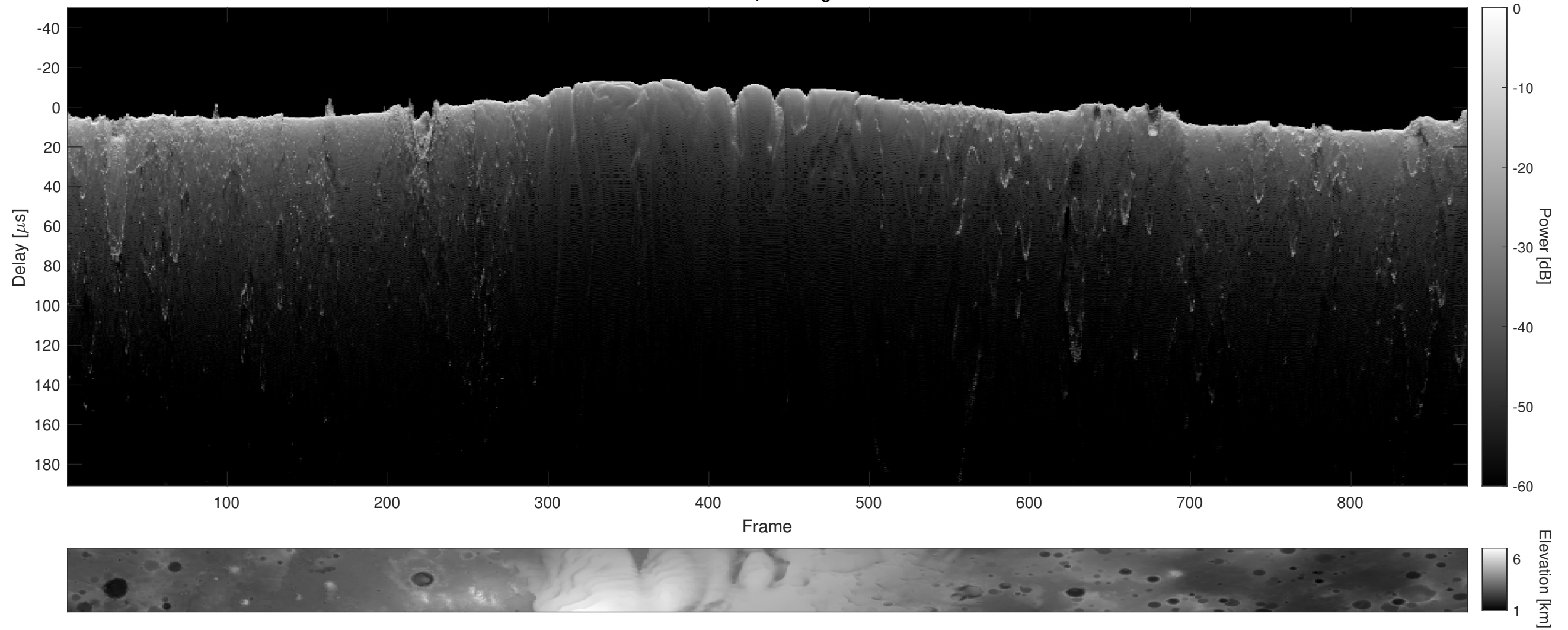
Orbit 8657, Cluttergram
