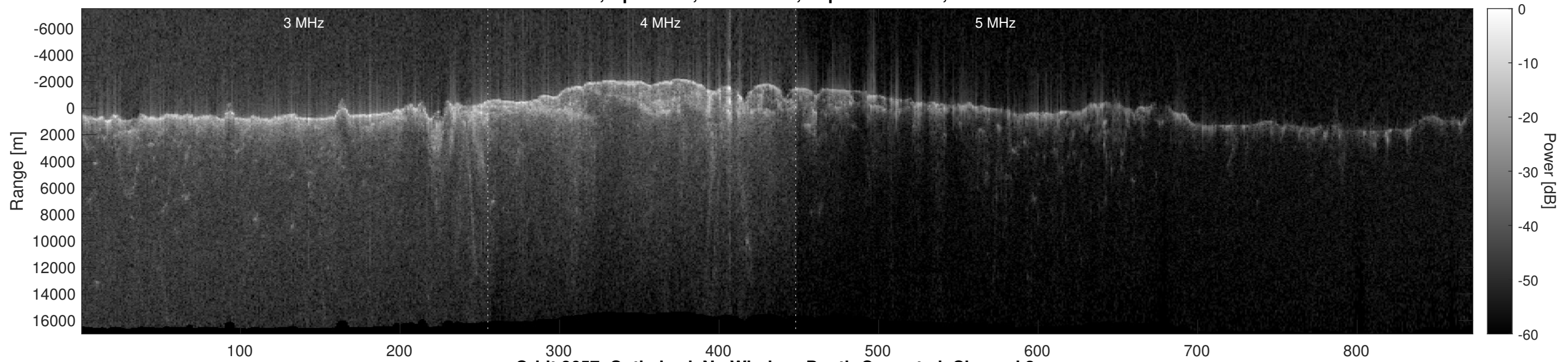
Orbit 8657, Optimized, No Window, Depth-Corrected, Channel 2
