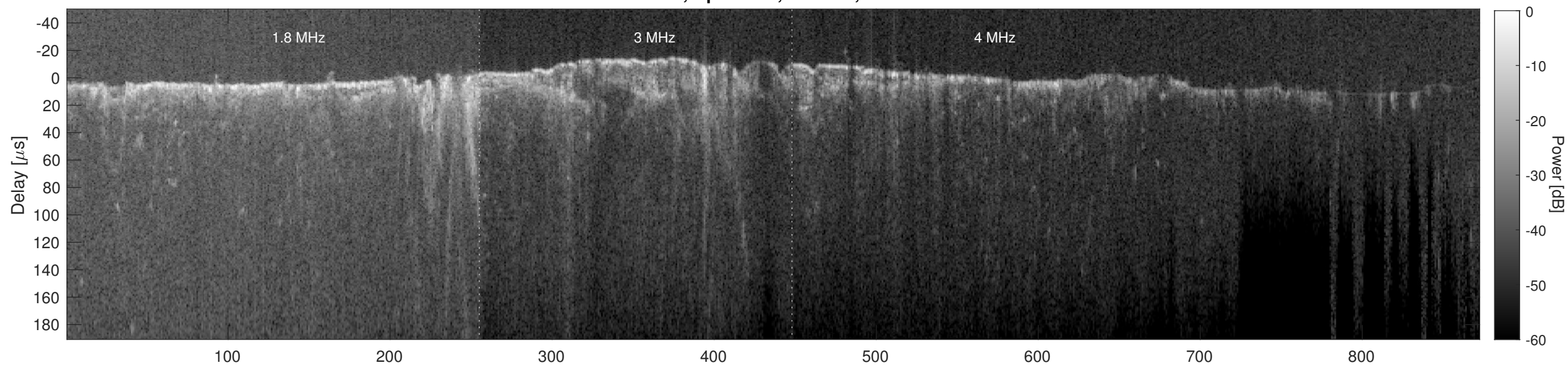
Orbit 8657, Cluttergram
