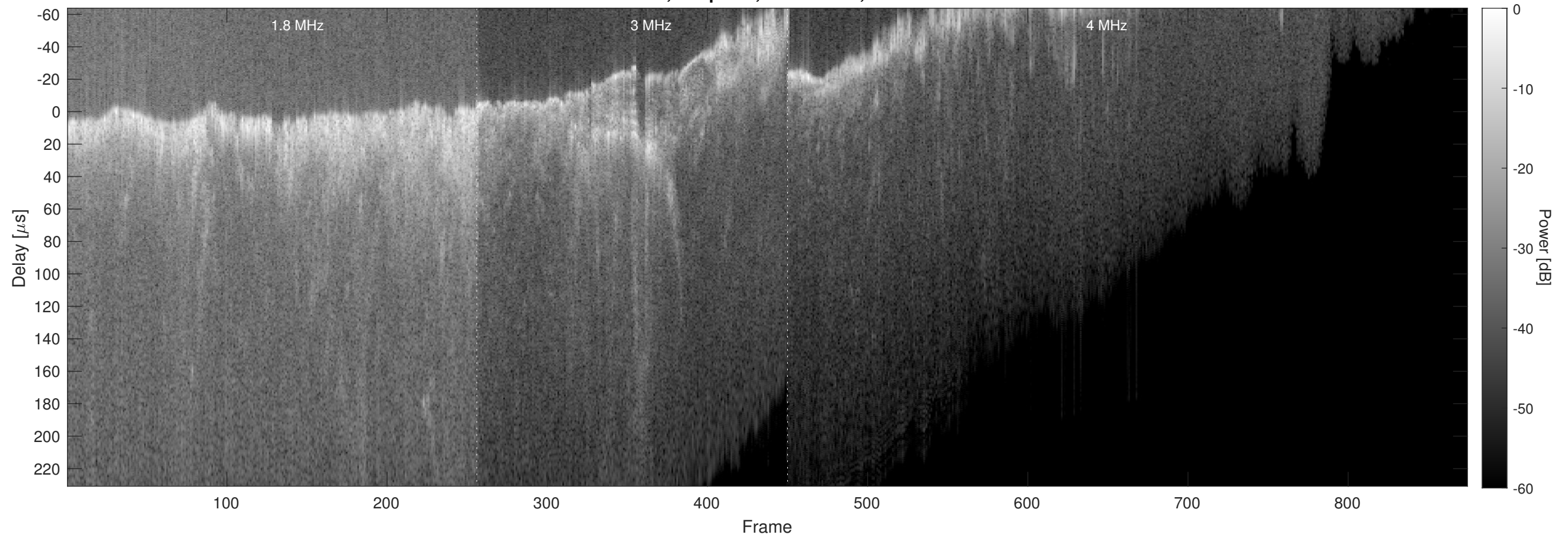
Orbit 8658, Chapman, No Window, Channel 2
