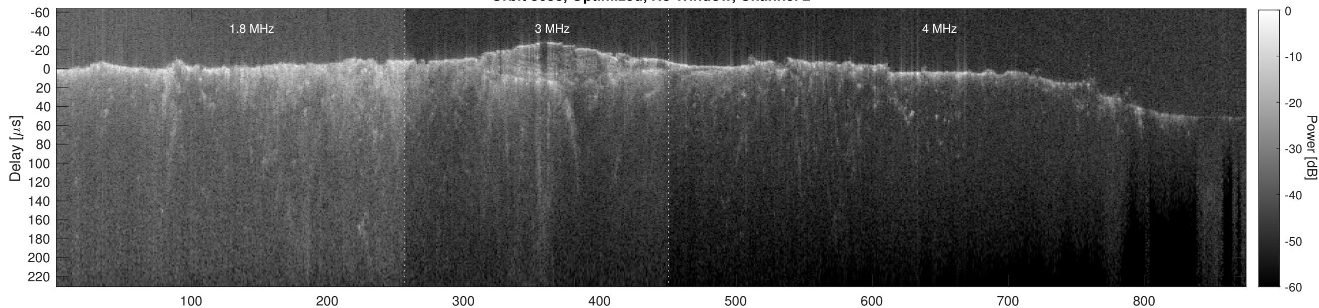
Orbit 8658, Cluttergram
