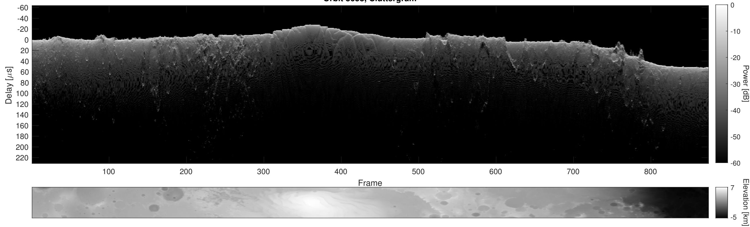
Orbit 8658, Cluttergram
