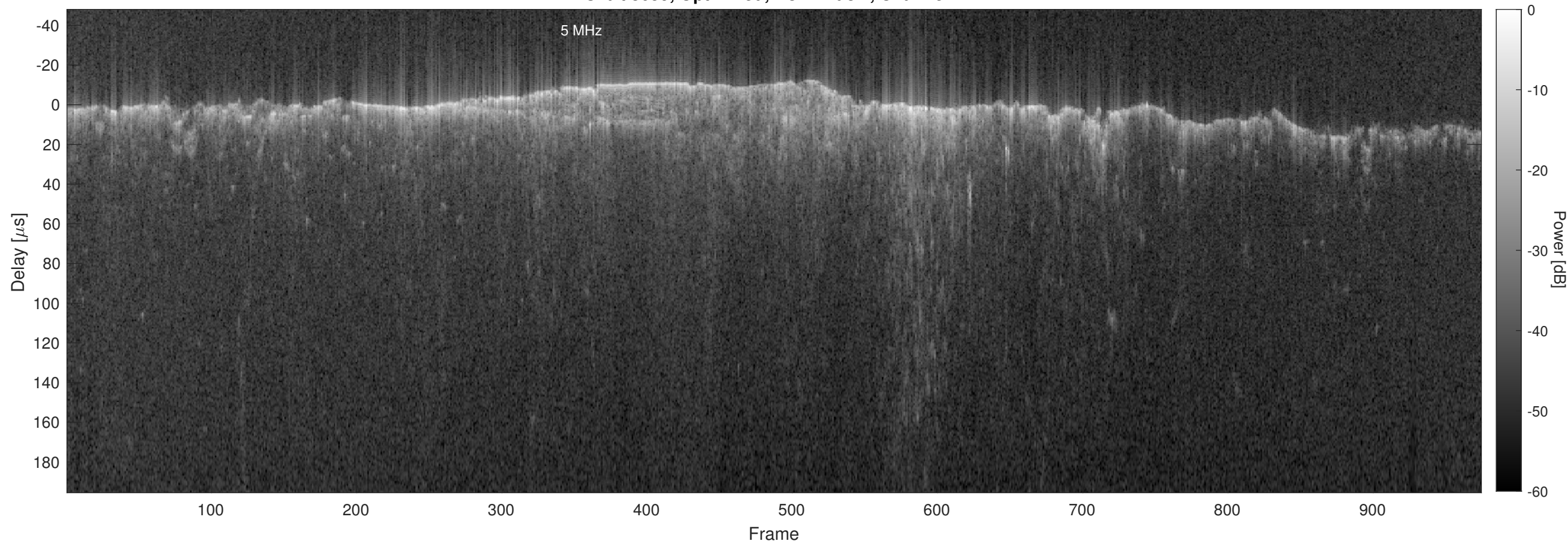
Orbit 8659, Optimized, No Window, Channel 2
