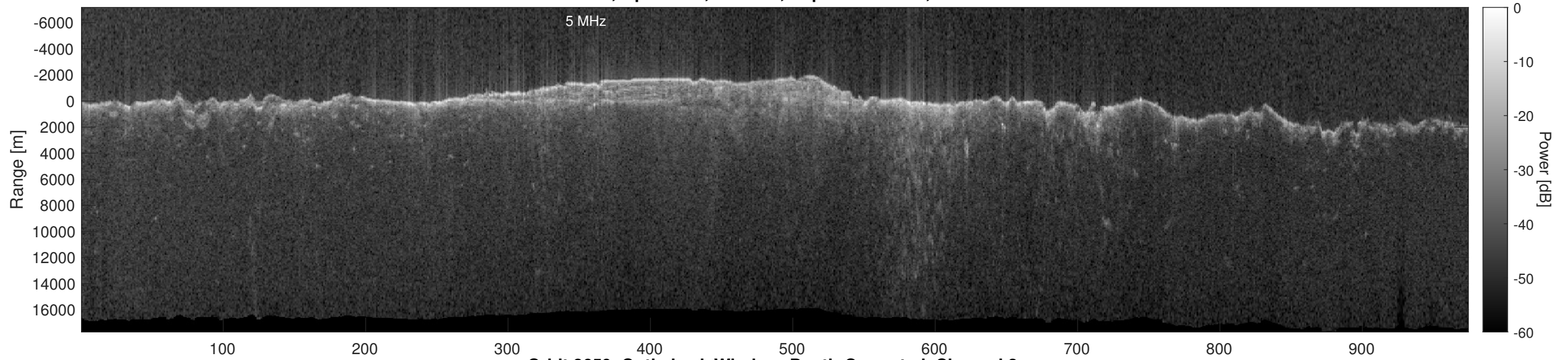
Orbit 8659, Optimized, Window, Depth-Corrected, Channel 2
