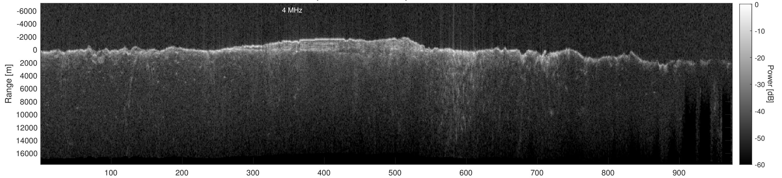
Orbit 8659, Depth-Corrected Cluttergram
