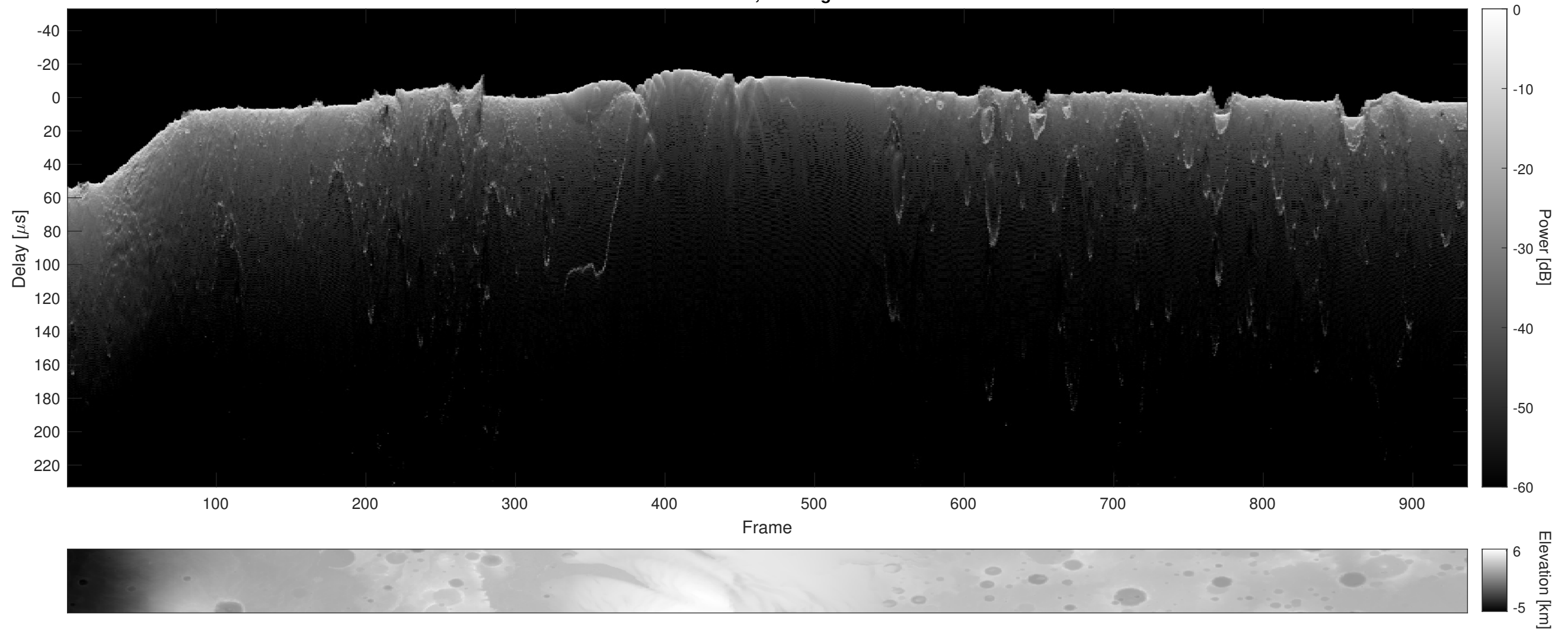
Orbit 8660, Cluttergram
