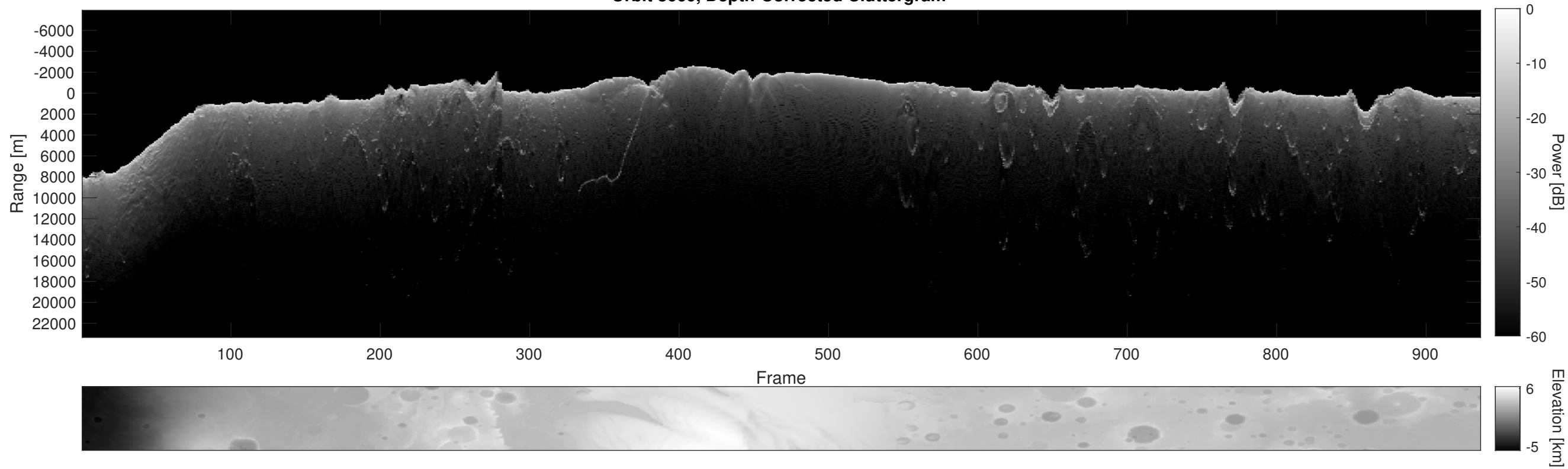
Orbit 8660, Depth-Corrected Cluttergram
