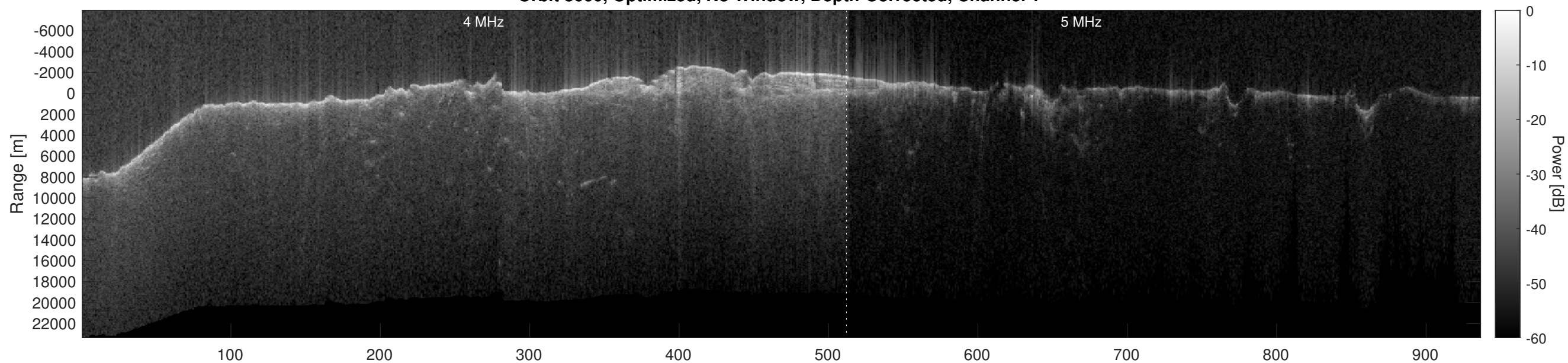
Orbit 8660, Optimized, No Window, Depth-Corrected, Channel 2
