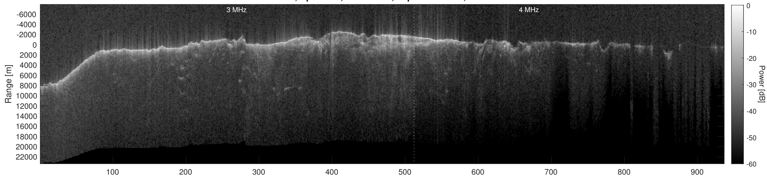
Orbit 8660, Depth-Corrected Cluttergram
