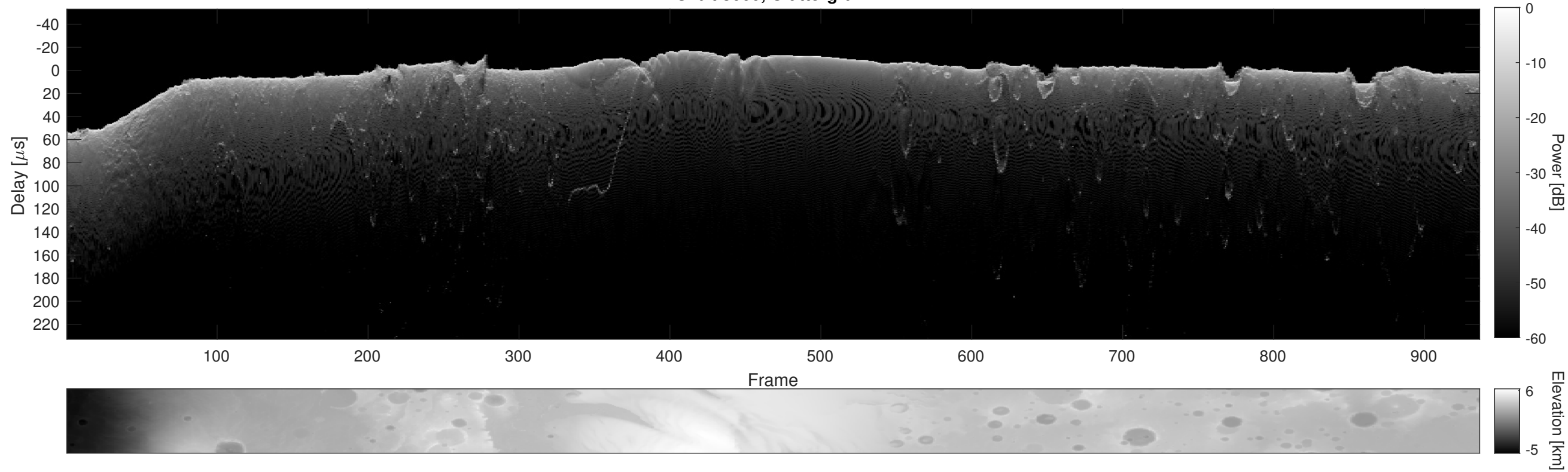
Orbit 8660, Cluttergram
