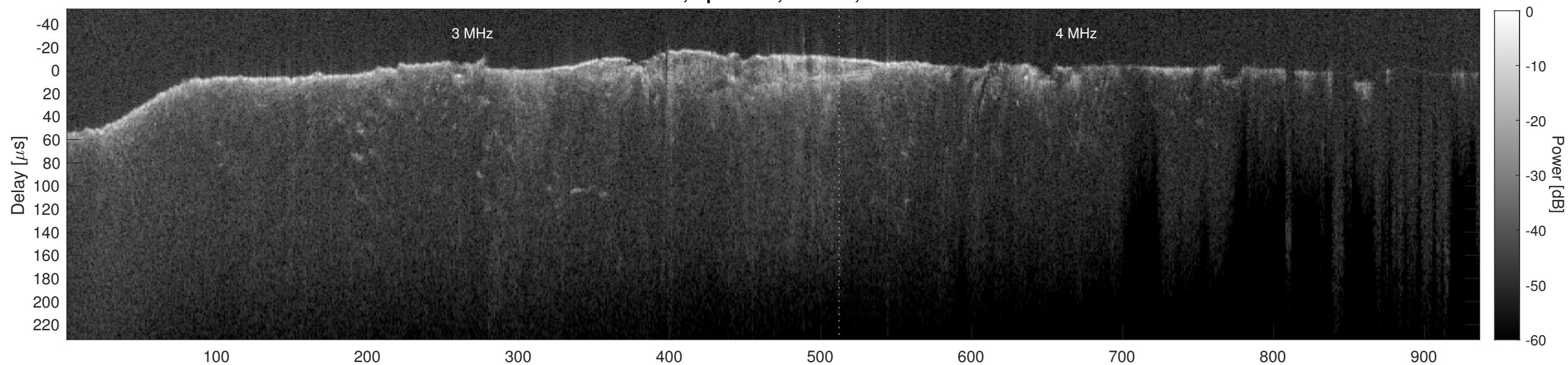
Orbit 8660, Cluttergram
