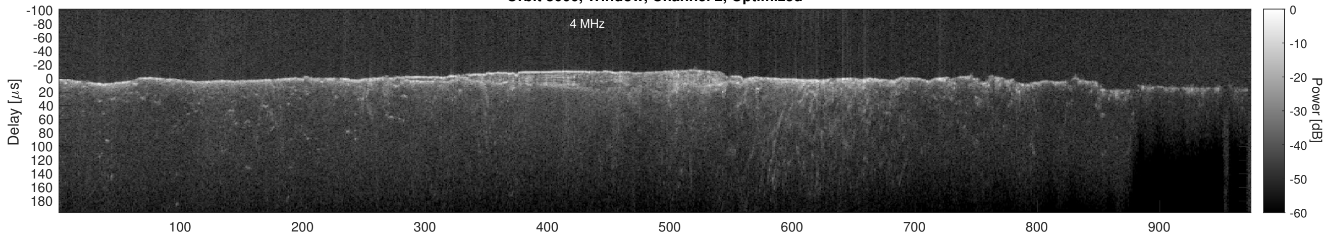
Orbit 8666, Cluttergram
