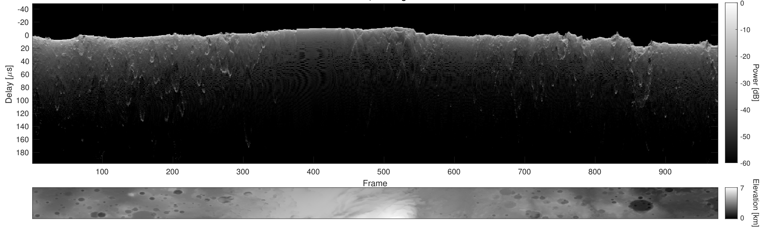
Orbit 8666, Cluttergram
