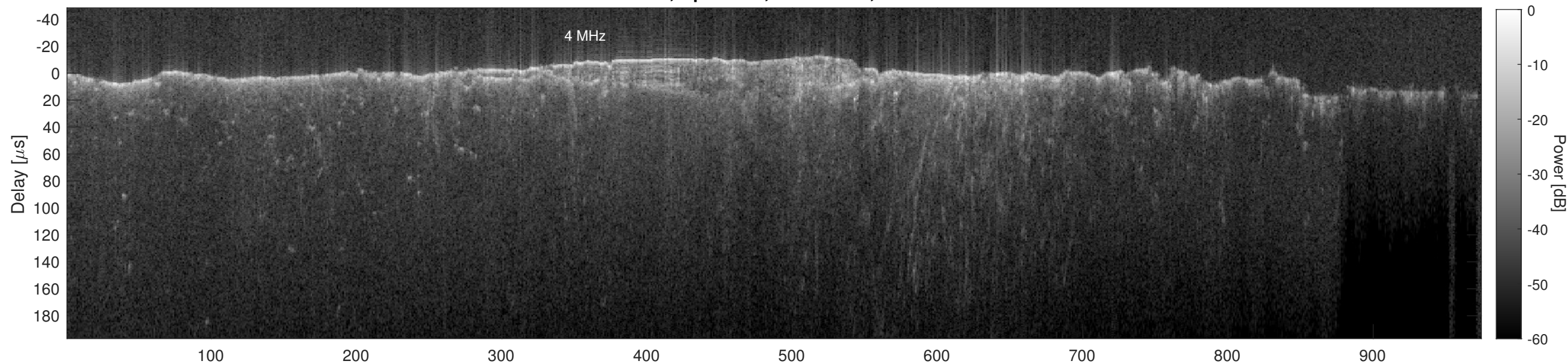
Orbit 8666, Cluttergram
