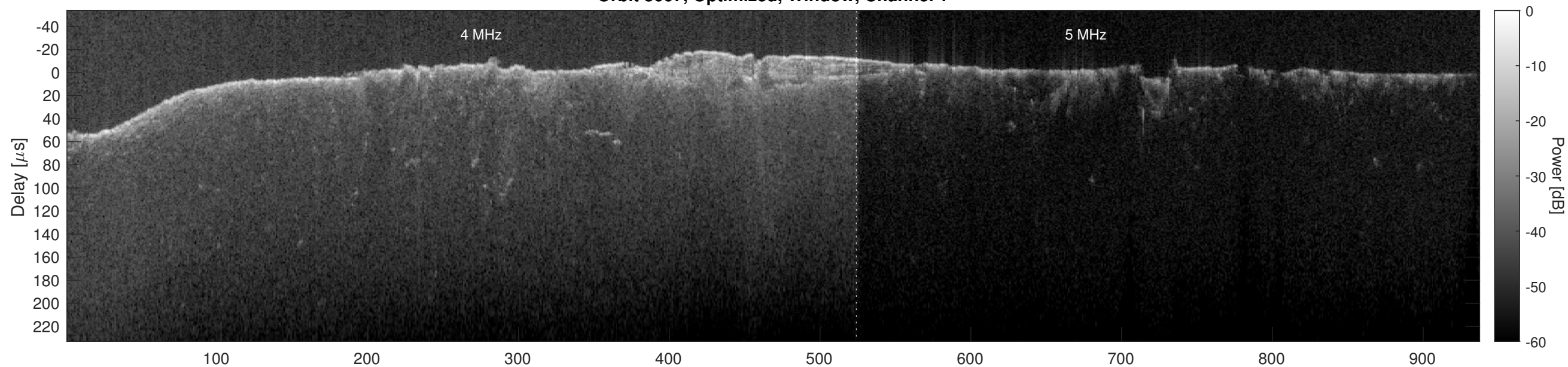
Orbit 8667, Optimized, Window, Channel 2
