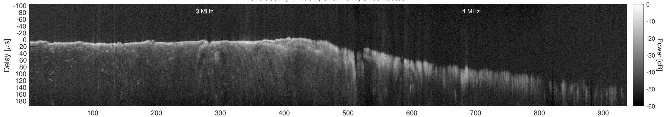
Orbit 8671, Window, Channel 2, Chapman
