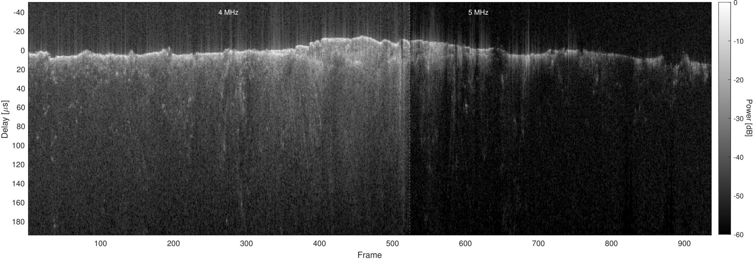
Orbit 8671, Optimized, No Window, Channel 2
