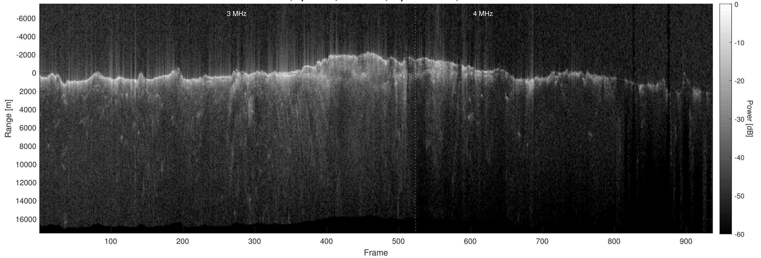
Orbit 8671, Optimized, No Window, Depth-Corrected, Channel 2
