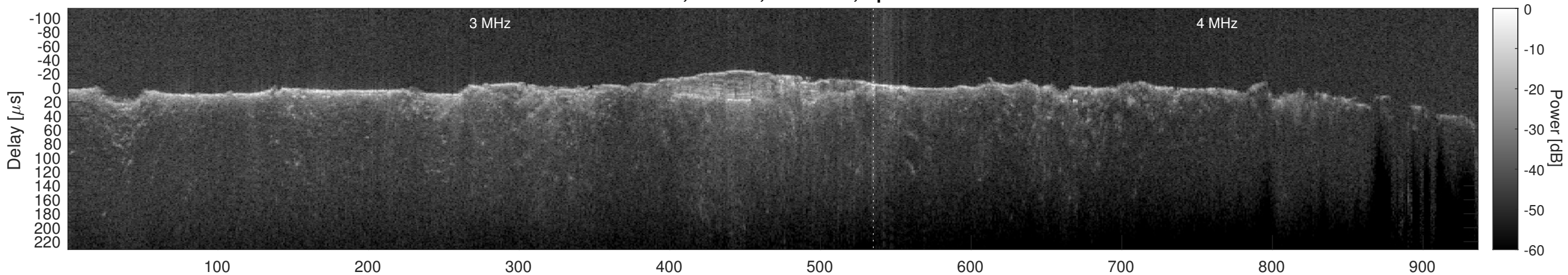
Orbit 8672, Cluttergram
