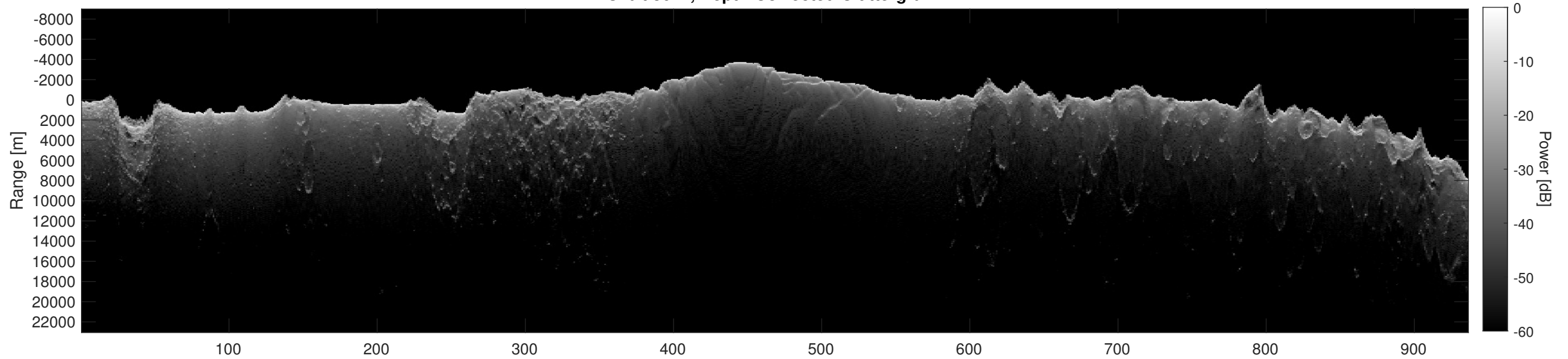
Orbit 8672, Depth-Corrected Cluttergram
