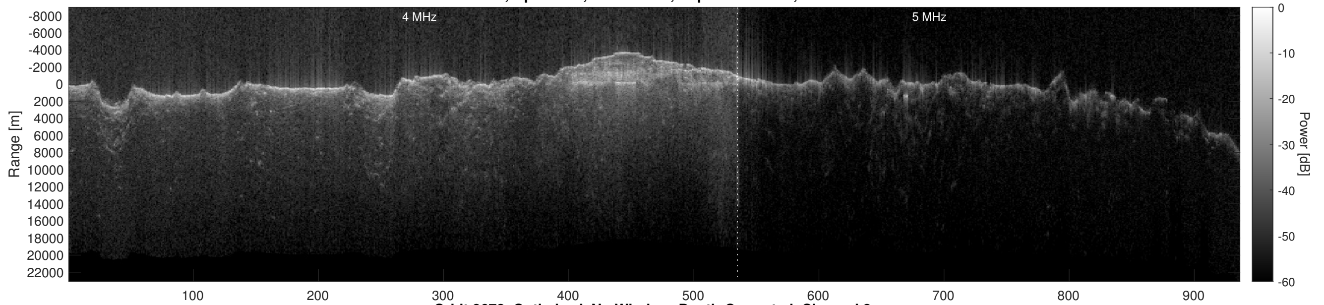
Orbit 8672, Optimized, No Window, Depth-Corrected, Channel 2
