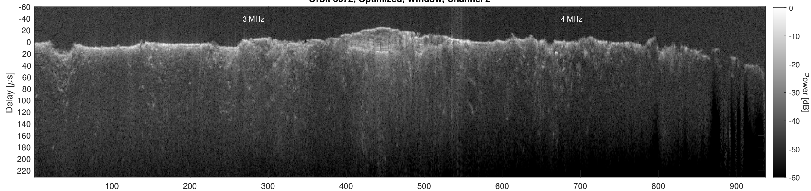
Orbit 8672, Cluttergram
