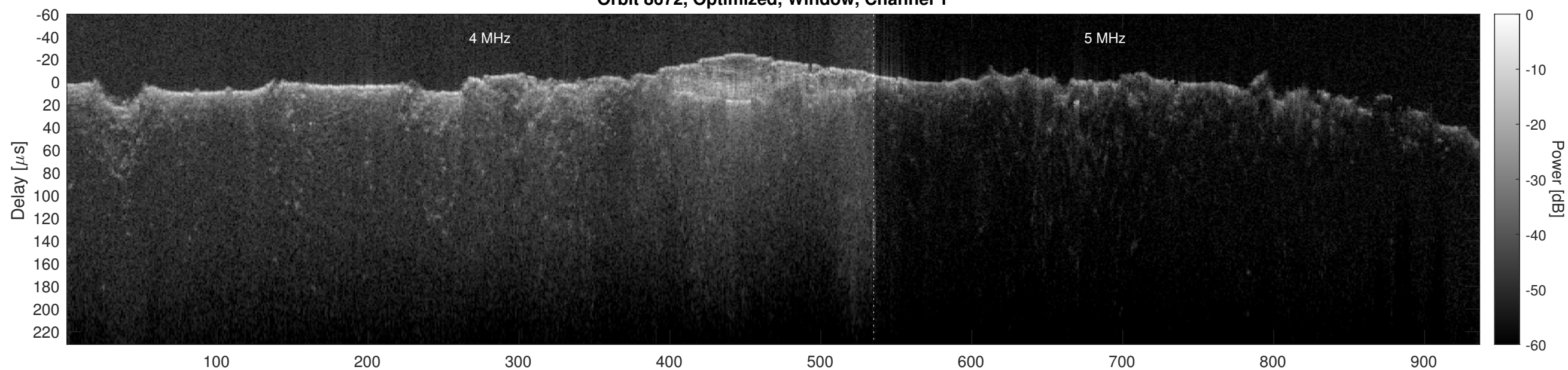
Orbit 8672, Optimized, Window, Channel 2
