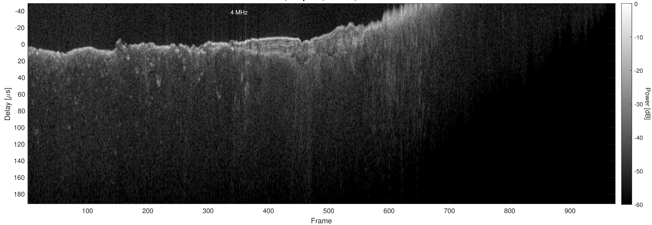
Orbit 8673, Chapman, Window, Channel 2
