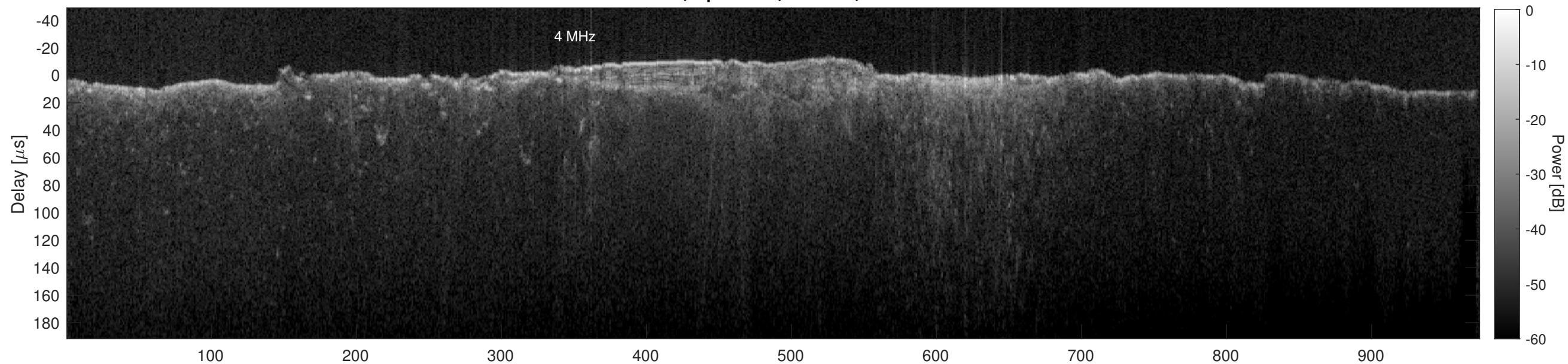
Orbit 8673, Cluttergram
