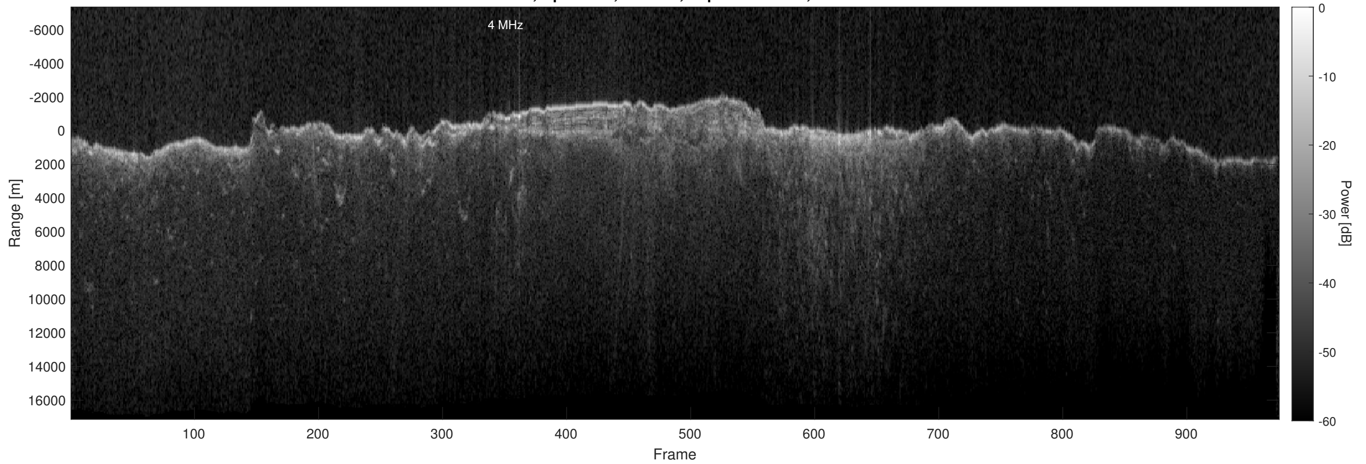
Orbit 8673, Optimized, Window, Depth-Corrected, Channel 2
