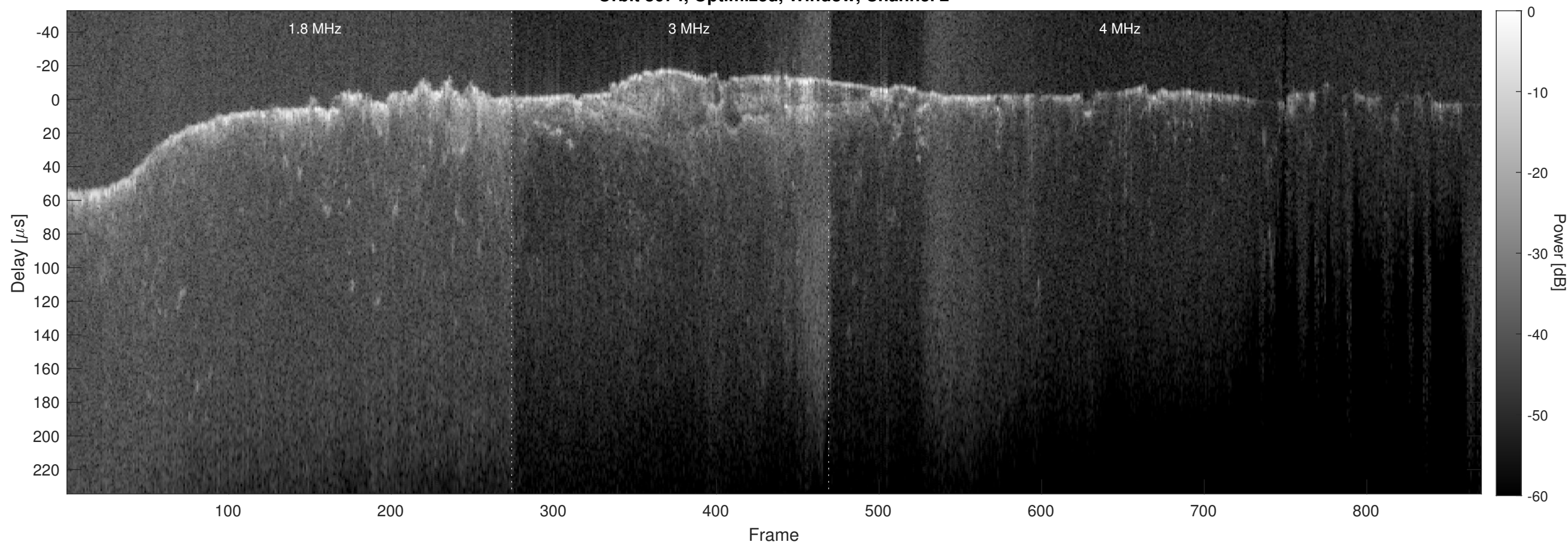
Orbit 8674, Optimized, Window, Channel 2
