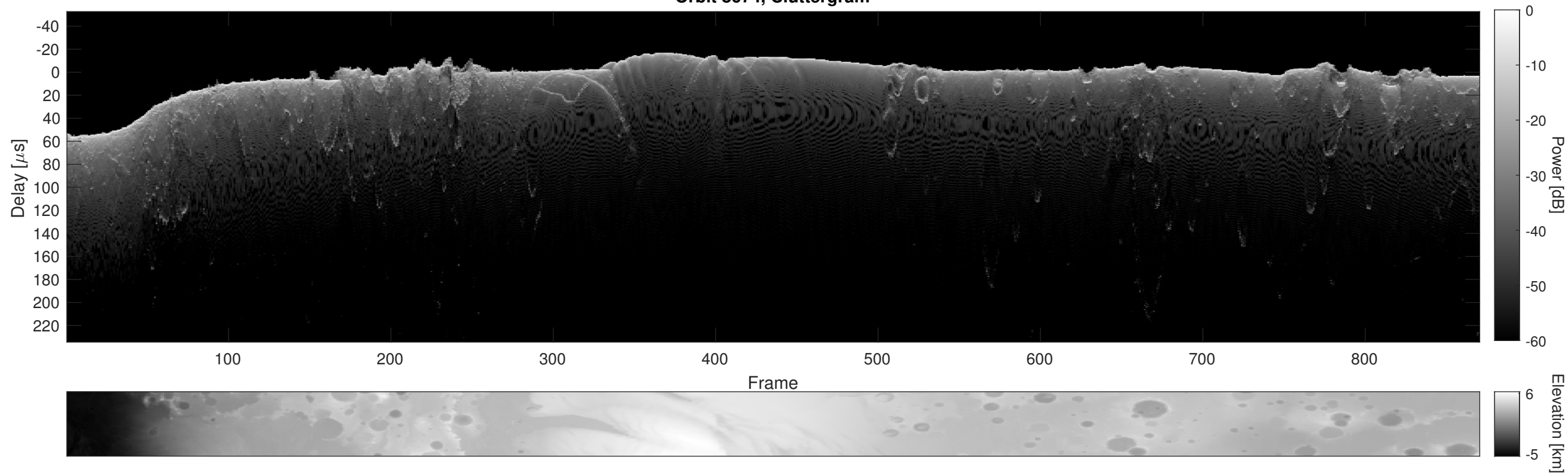
Orbit 8674, Cluttergram
