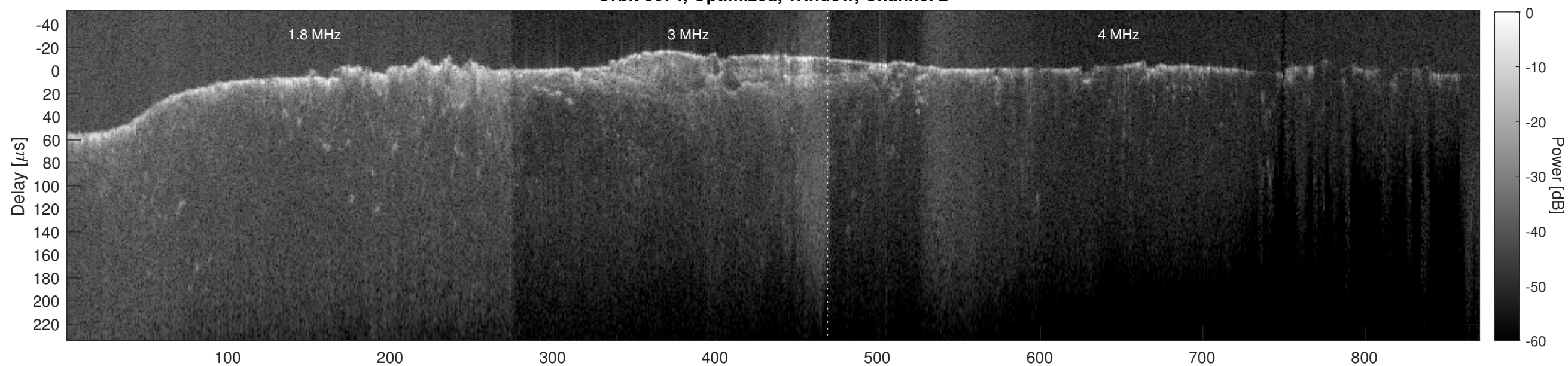
Orbit 8674, Cluttergram
