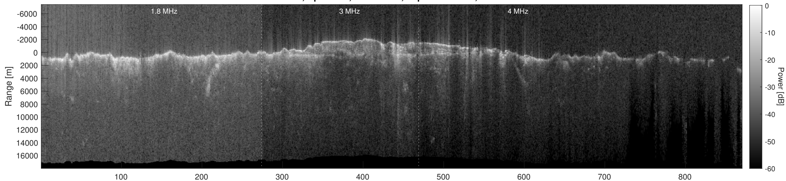
Orbit 8678, Depth-Corrected Cluttergram
