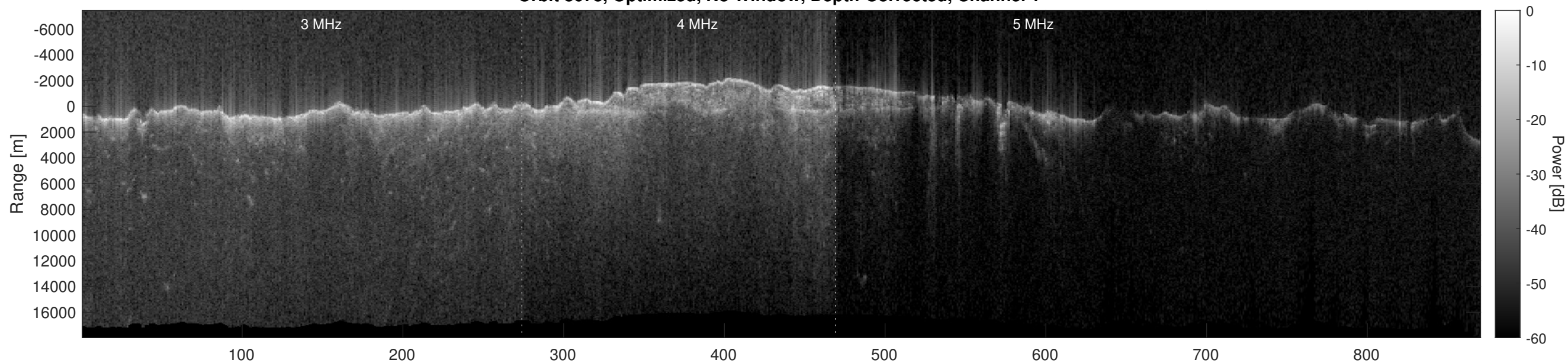
Orbit 8678, Optimized, No Window, Depth-Corrected, Channel 2
