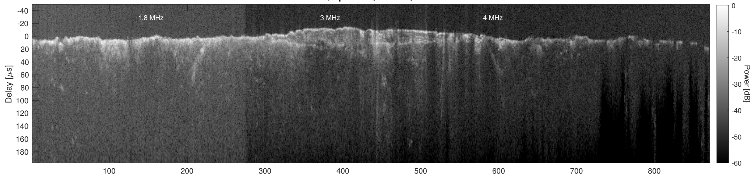
Orbit 8678, Cluttergram
