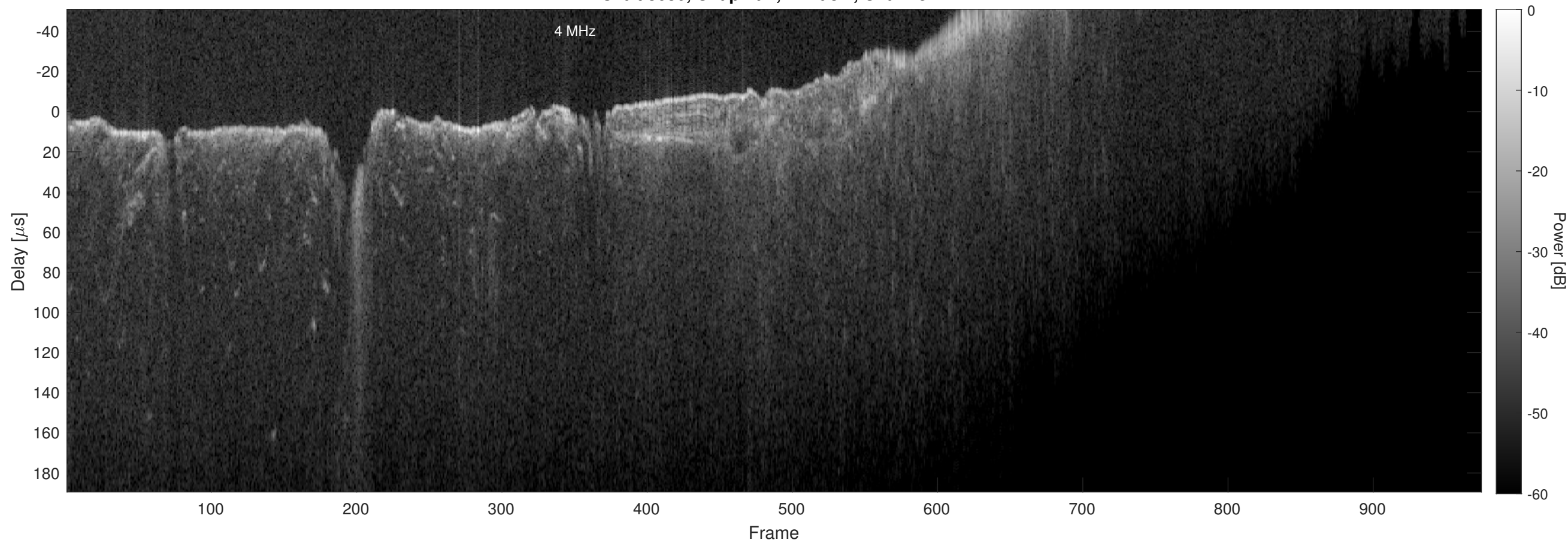
Orbit 8680, Chapman, Window, Channel 2
