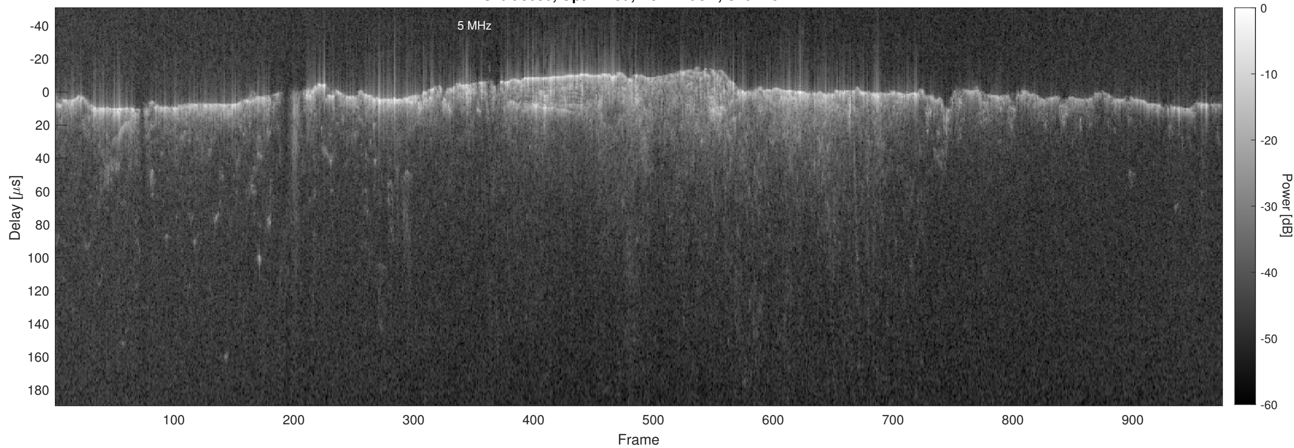
Orbit 8680, Optimized, No Window, Channel 2
