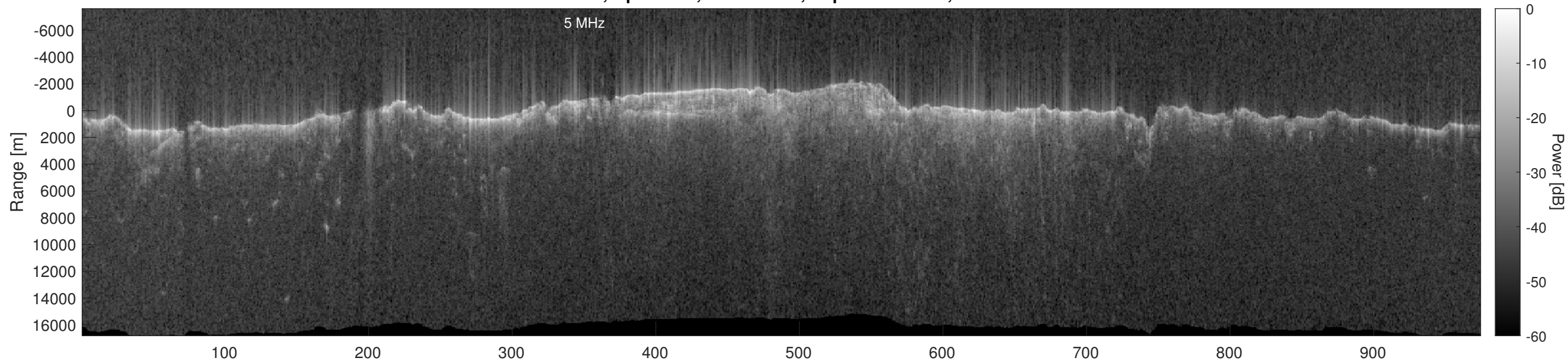
Orbit 8680, Optimized, No Window, Depth-Corrected, Channel 2
