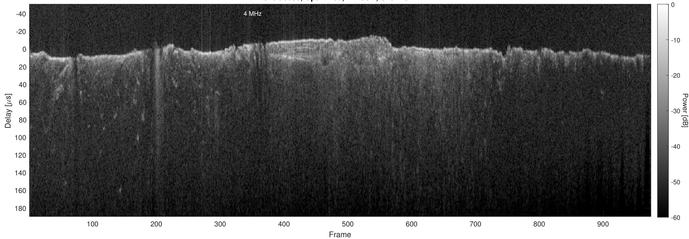
Orbit 8680, Optimized, Window, Channel 2
