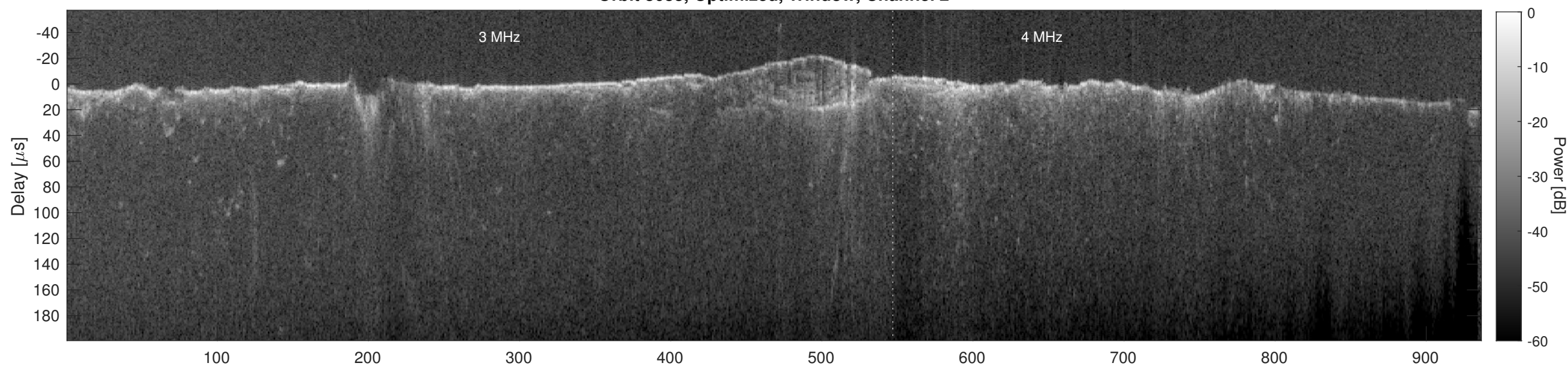
Orbit 8683, Cluttergram
