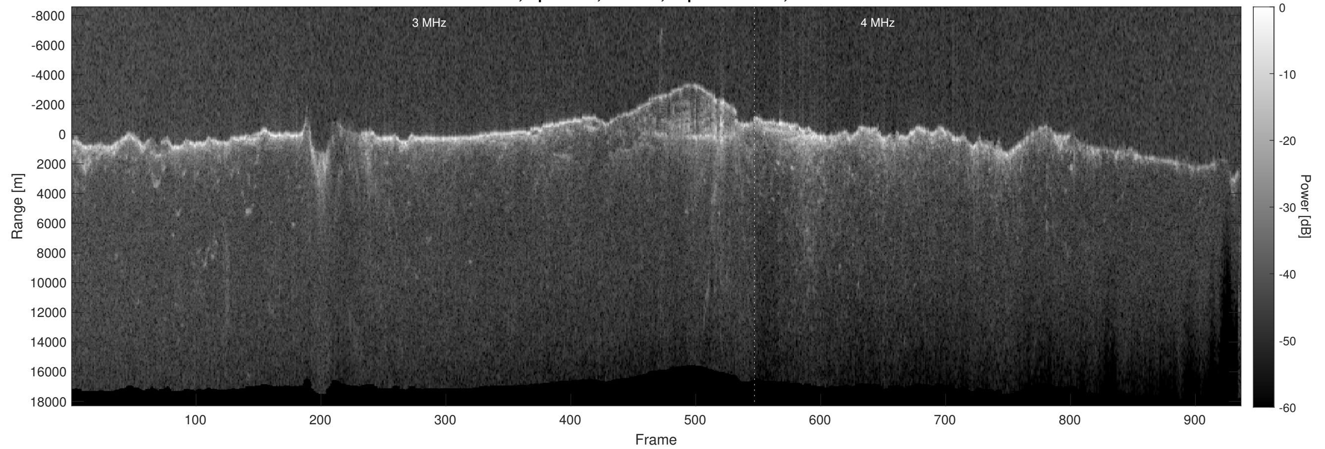
Orbit 8683, Optimized, Window, Depth-Corrected, Channel 2
