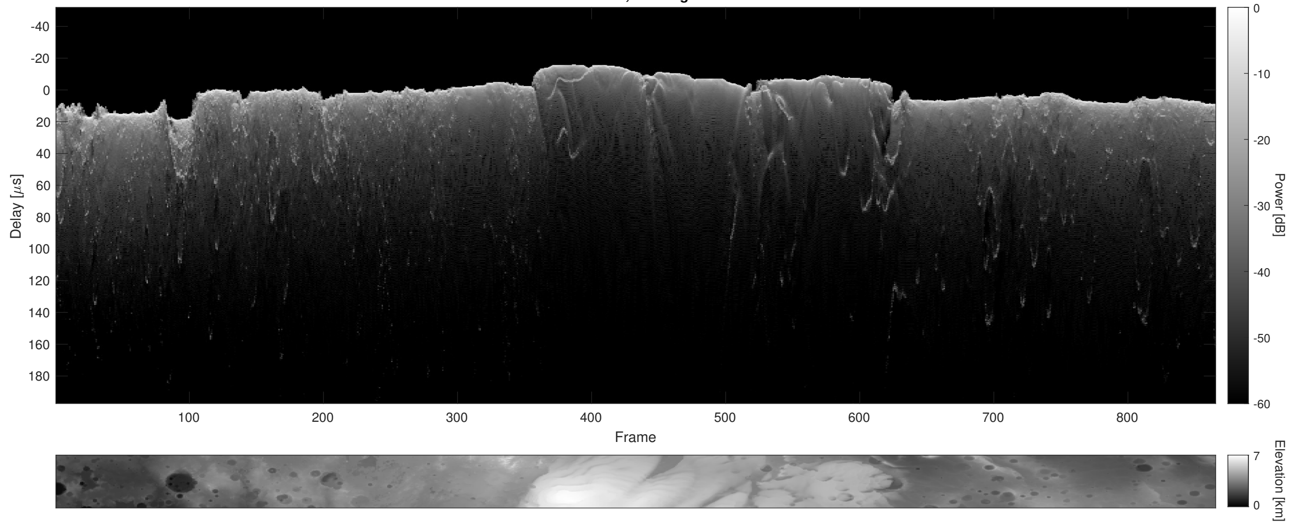
Orbit 8689, Cluttergram
