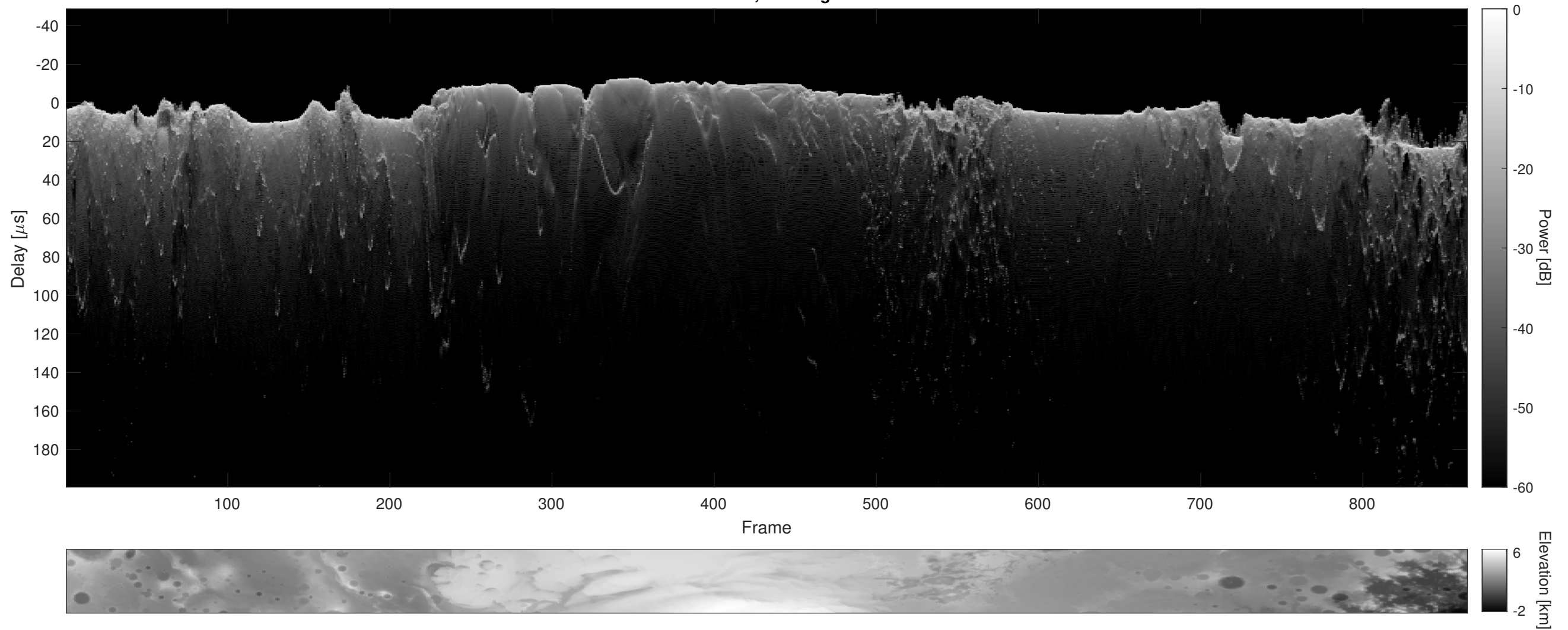
Orbit 8691, Cluttergram
