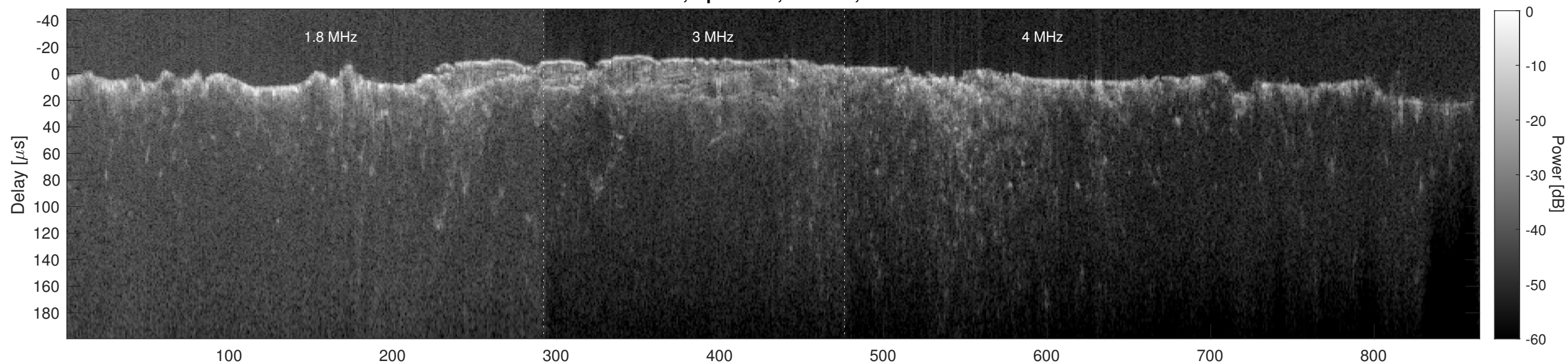
Orbit 8691, Cluttergram
