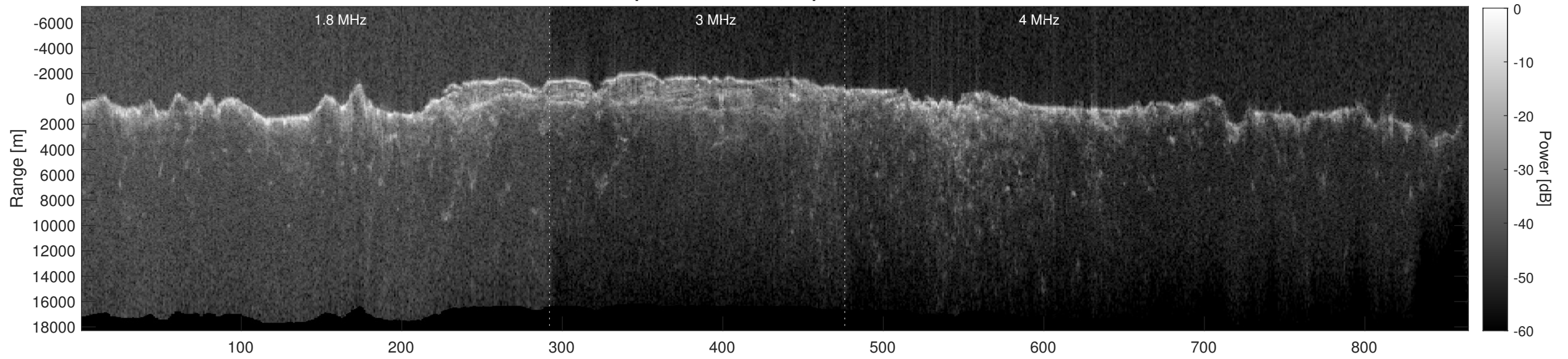
Orbit 8691, Depth-Corrected Cluttergram
