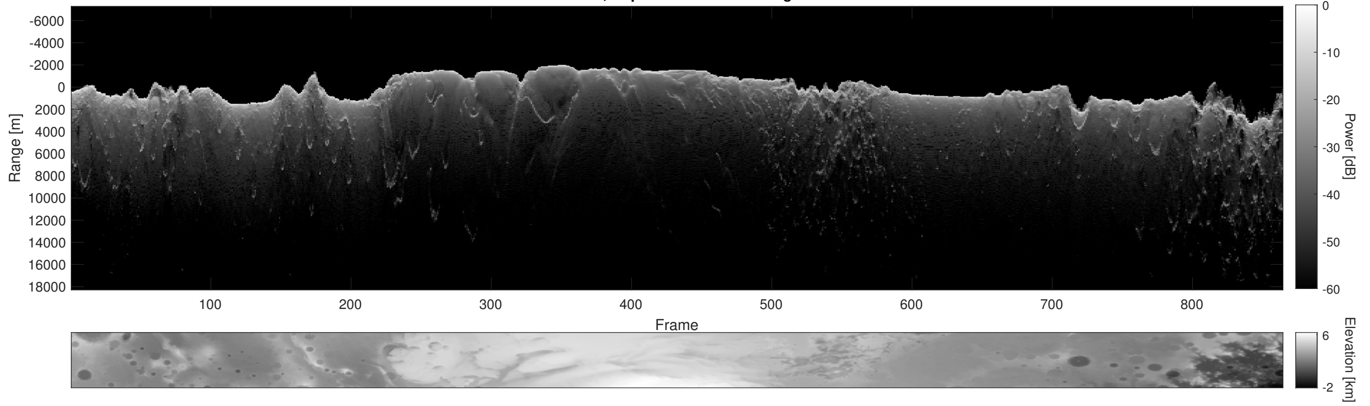
Orbit 8691, Depth-Corrected Cluttergram
