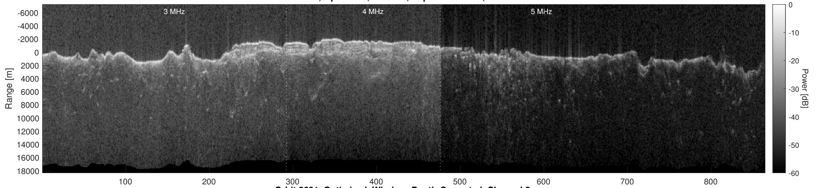
Orbit 8691, Optimized, Window, Depth-Corrected, Channel 2
