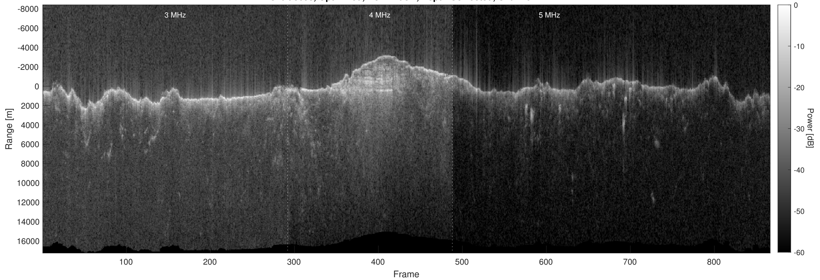
Orbit 8693, Optimized, No Window, Depth-Corrected, Channel 2
