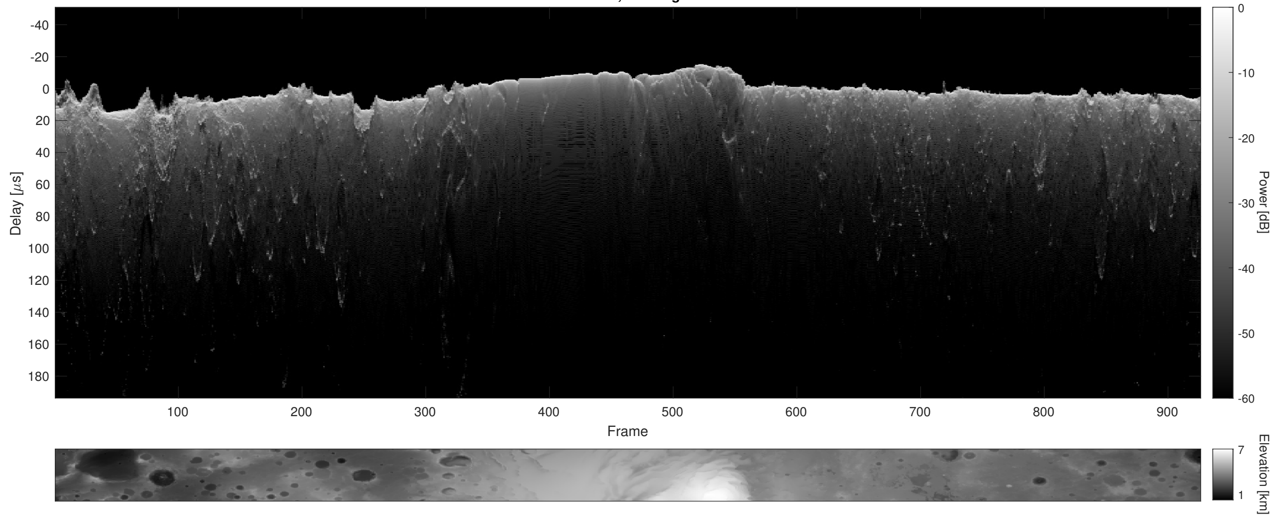
Orbit 8694, Cluttergram
