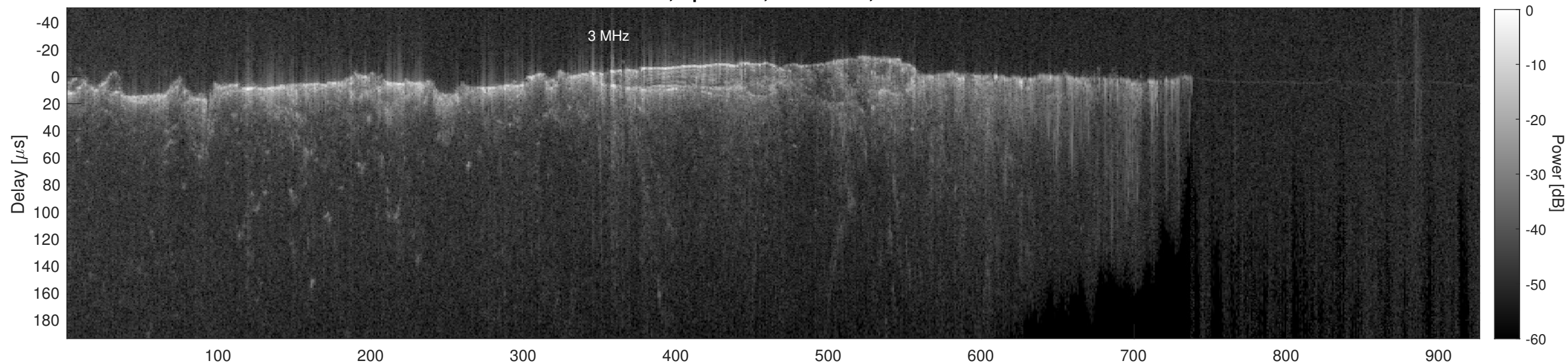
Orbit 8694, Cluttergram
