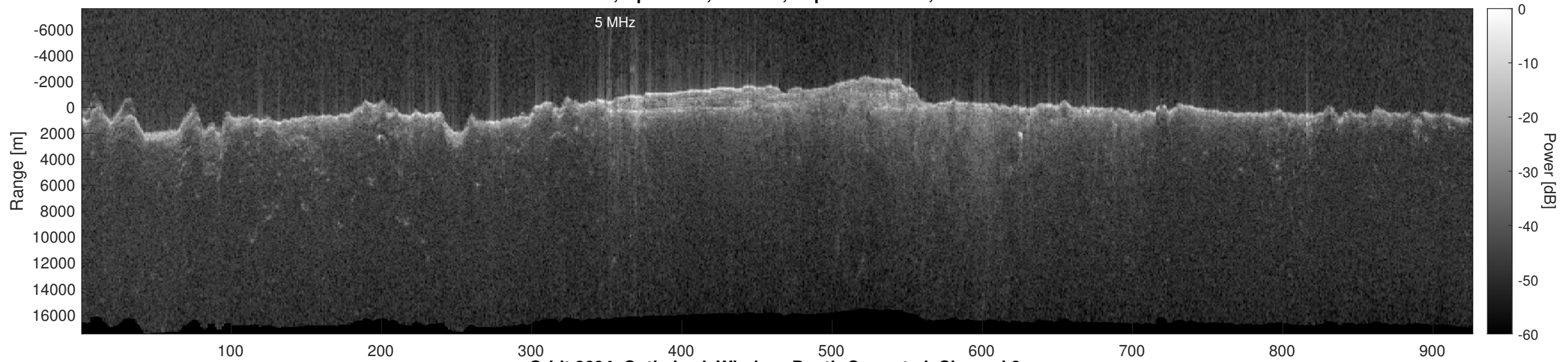
Orbit 8694, Optimized, Window, Depth-Corrected, Channel 2
