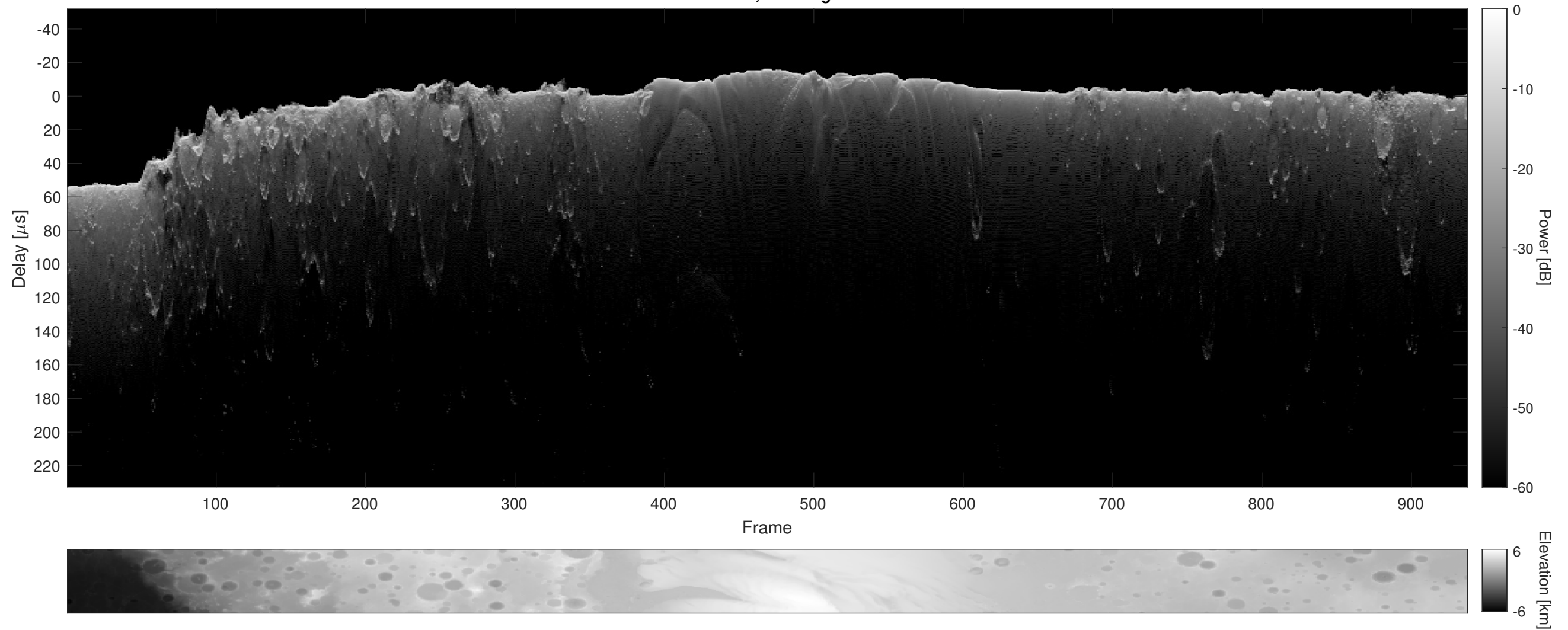
Orbit 8695, Cluttergram
