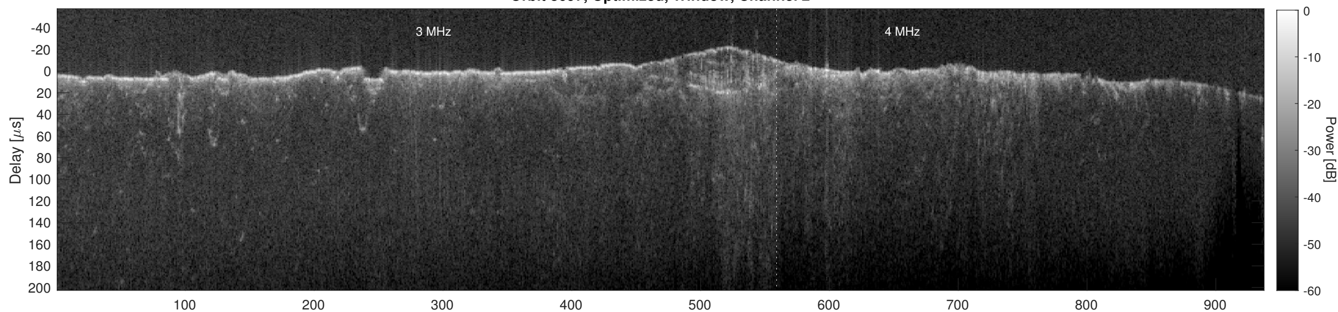
Orbit 8697, Cluttergram
